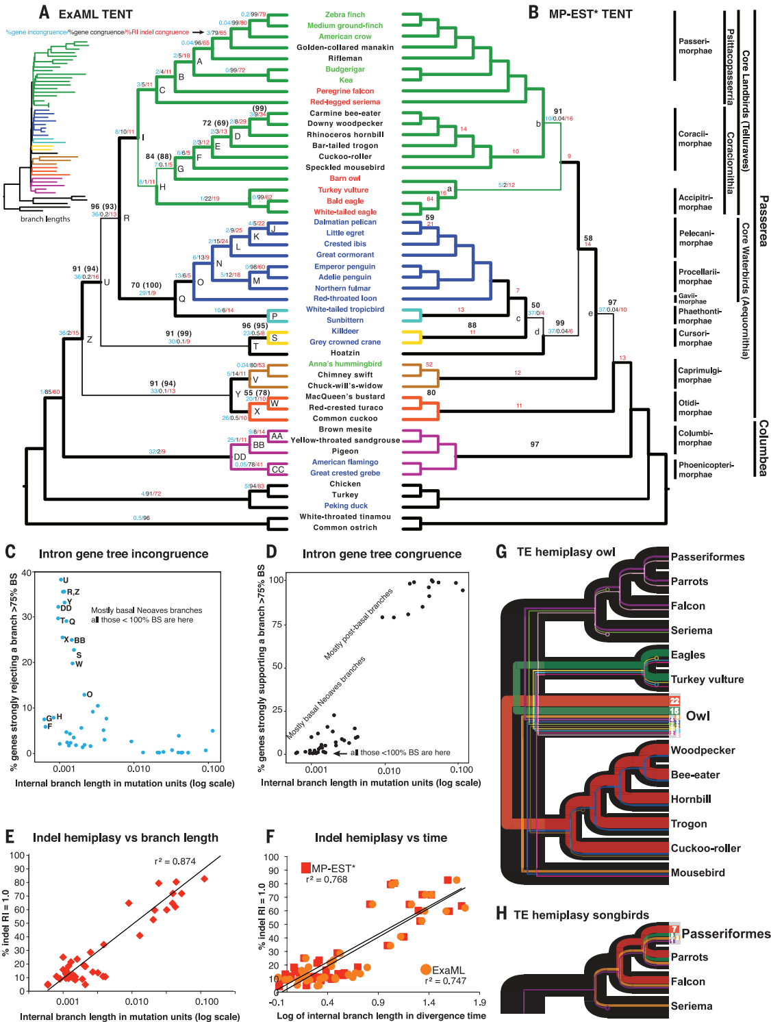
Fig. 3. Evidence of ILS. (A) Cladogram of ExaML TENT avian species tree, annotated for nodes from Fig. 2 (letters), for branches with less than 100% BS without and with (parentheses) third codon positions, for strong (>75% BS) intron gene tree incongruence and congruence, and for indel congruence on all branches (except the root). Thin branch lines represent those not present in the MP-EST* TENT of (B). (Inset) ExaML branch lengths in substitution units (expanded view in fig. S7). Color coding of branches and species is as in Fig. 1. (B) Cladogram of MP-EST* TENT species tree, annotated similarly as in the ExaML TENT in (A). Thin branch lines represent those not present in the ExaML TENT of (A). (C) Percent of intron gene trees rejecting ( \geq 75\% BS) branches in the ExaML TENT species tree relative to branch lengths. Letters denote nodes in (A) that either have less than 100% support or are different from the MP-EST* TENT in (B). (D) Percent of intron gene trees supporting ( \geq 75\% BS) branches in the ExaML TENT species tree relative to branch lengths. (E) Indel hemiplasy [the inverse of percent of retention index (RI) = 1.0 indels that support the branch; see SM9] correlated with ExaML TENT branch length (log transformed). r^2 , correlation coefficient. (F) Indel hemiplasy correlated with ExaML and MP-EST TENT internal branch divergence times in millions of years (log transformed). Plotting with internal branch times was necessary to compare both trees (SM9). (G) TE hemiplasy with owls among the core landbirds. Line color, shared TE tree topology; line thickness, relative proportion of TEs that support a specific topology (total numbers shown in the owl node). Circles at end of lines indicate loss of the TE allele in that species after ILS, as the sequence assembly contains an empty TE insertion site (SM10). Only topologies with two or more TEs are shown. (H) TE hemiplasy with songbirds among the core landbirds.
